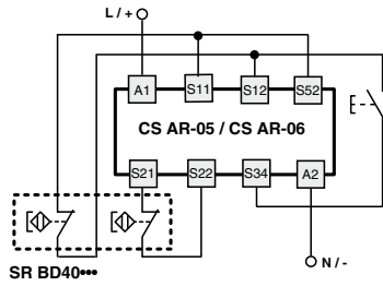
Input configuration with manual start (CS AR-05) and monitored start (CS AR-06) 2 channels
