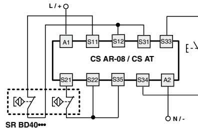
Input configuration with manual start 2 channels
